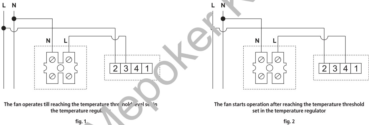
Temperature regulator connection options
